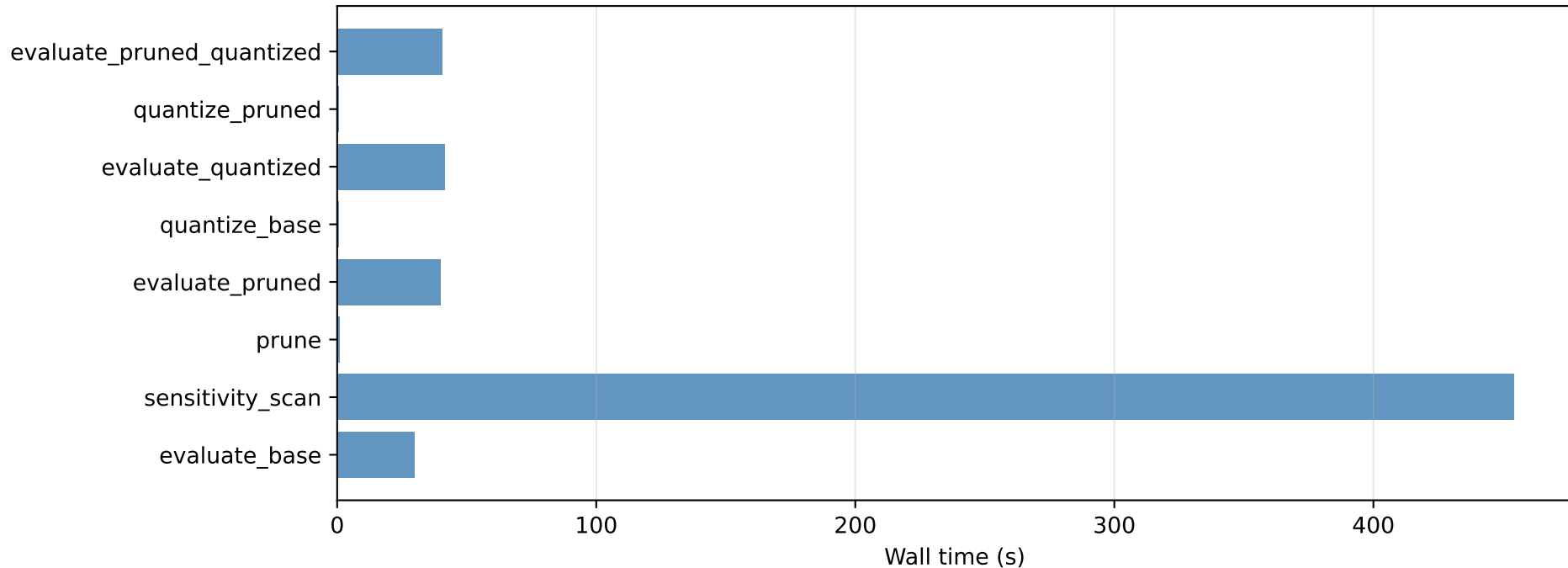
Benchmark — distilgpt2-wikitext
