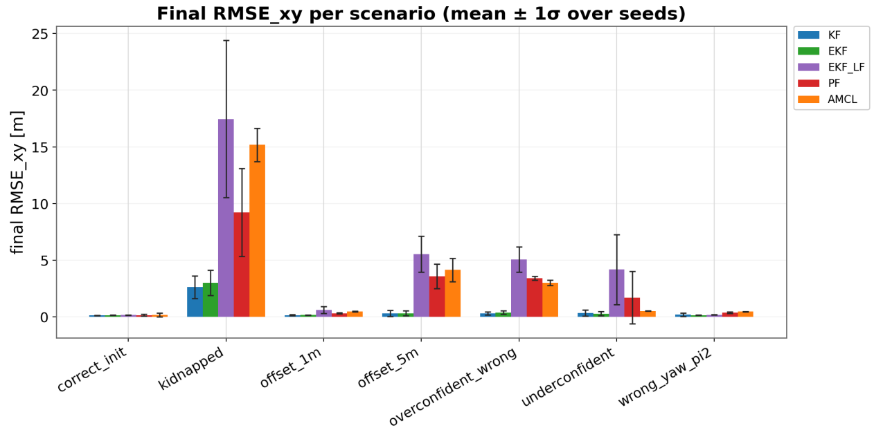
Fig. 3: Final \text{RMSE}_{xy} per scenario (mean \pm 1\sigma , ten seeds). The landmark filters (KF, EKF) remain low across every adverse scenario; the scan filters explode under offset_5m, overconfident_wrong, and kidnapped.
