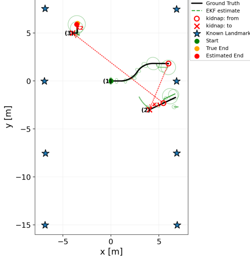
(a) EKF (landmark): recovers.
