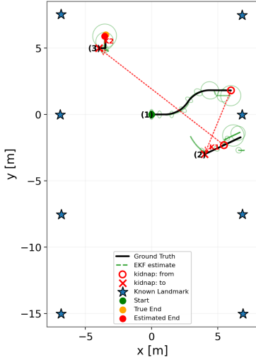
(a) EKF (landmark): recovers.
