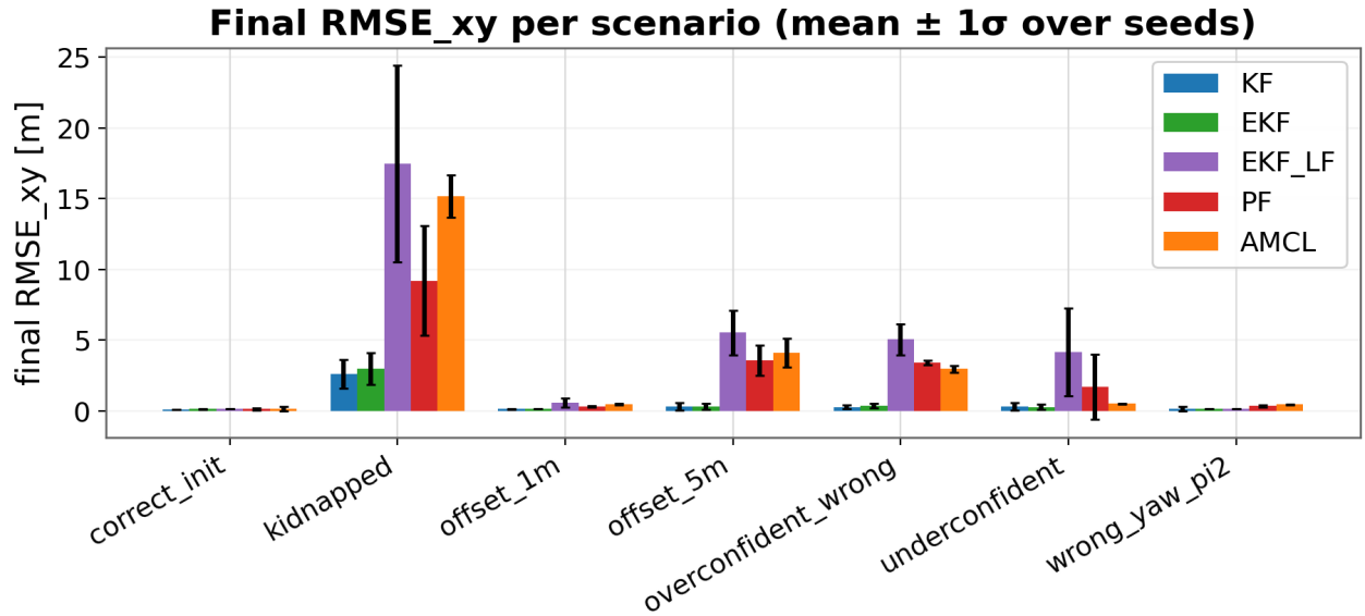
Fig. 2: Final RMSE_{xy} per scenario (mean \pm 1\sigma , ten seeds). The landmark filters (KF, EKF) remain low across every adverse scenario; the scan filters explode under offset_5m , overconfident_wrong , and kidnapped .
