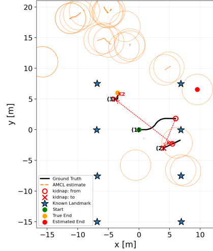
(b) AMCL (scan): diverges.
