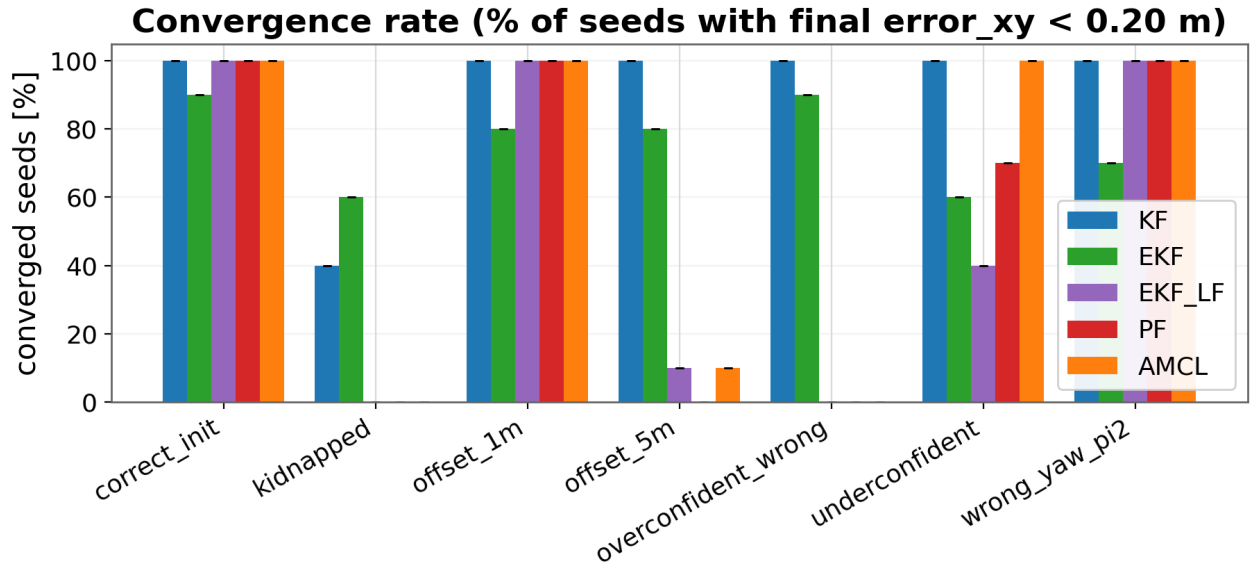
Fig. 4: Convergence rate: percentage of seeds whose final position error is below 0.20 m. The landmark filters succeed in the adverse scenarios where the scan filters never converge; the partial kidnap recovery (40–60%) reflects the stochastic search through the aliased map.
