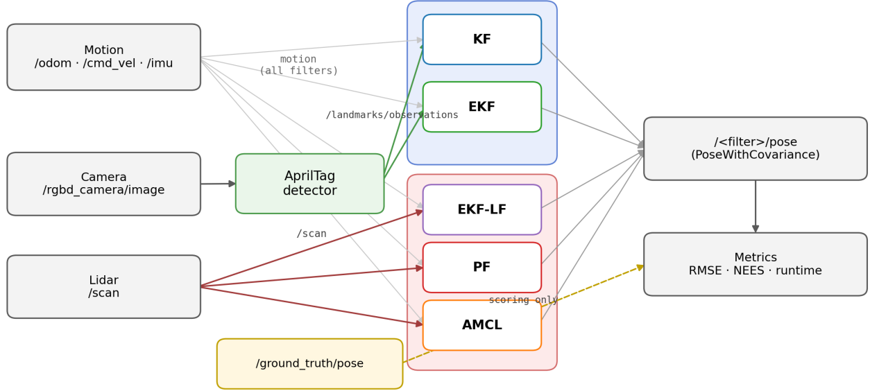
Fig. 1: System data flow. Wheel odometry, /cmd_vel and the IMU drive every filter’s motion model; the camera image is turned by the AprilTag detector into /landmarks/observations consumed by the landmark filters (KF, EKF), while /scan drives the scan filters (EKF-LF, PF, AMCL). Each filter publishes /<filter>/pose ; ground truth feeds the metrics only, never a filter.
