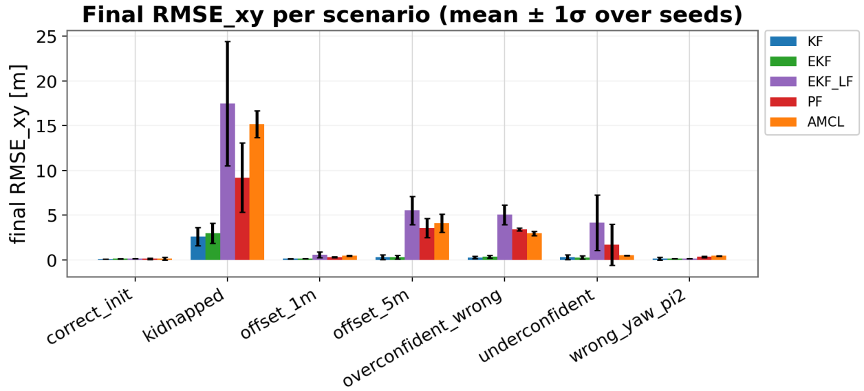
Fig. 3: Final RMSE xy per scenario (mean \pm 1\sigma , ten seeds). The landmark filters (KF, EKF) remain low across every adverse scenario; the scan filters explode under offset_5m , overconfident_wrong , and kidnapped .
