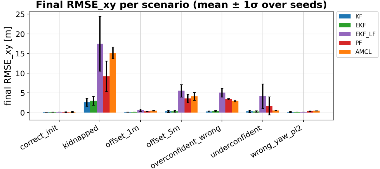
Fig. 3: Final \text{RMSE}_{xy} per scenario (mean \pm 1\sigma , ten seeds). The landmark filters (KF, EKF) remain low across every adverse scenario; the scan filters explode under offset_5m , overconfident_wrong , and kidnapped .
