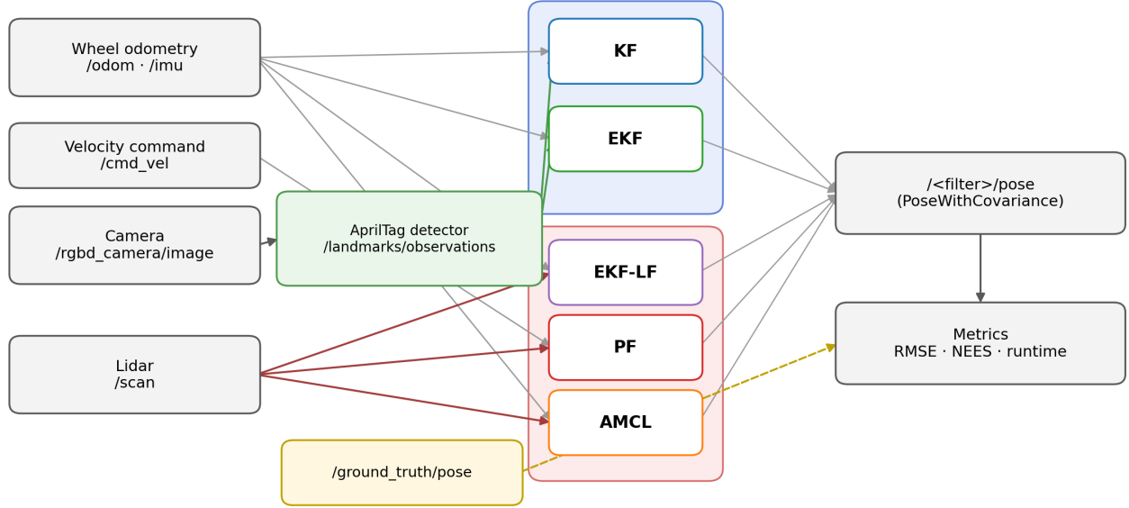
Fig. 1: System data flow. Wheel odometry ( /odom ) and the IMU drive the motion model of KF, EKF and EKF-LF (and AMCL via TF); the PF instead uses the /cmd_vel velocity command. The camera image is turned by the AprilTag detector into /landmarks/observations , consumed by the landmark filters (KF, EKF), while /scan drives the scan filters (EKF-LF, PF, AMCL). Each filter publishes /<filter>/pose ; ground truth feeds the metrics only, never a filter.
