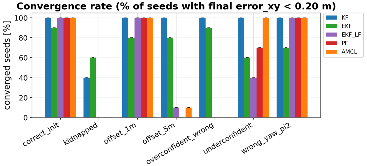
Fig. 5: Convergence rate: percentage of seeds whose final position error is below 0.20 m. The landmark filters succeed in the adverse scenarios where the scan filters never converge; the partial kidnap recovery (40–60%) reflects the stochastic search through the aliased map.
