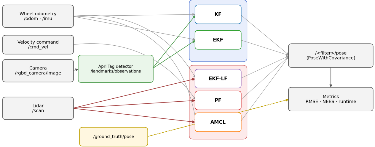
Fig. 1: System data flow. Wheel odometry ( /odom ) and the IMU drive the motion model of KF, EKF and EKF-LF (and AMCL via TF); the PF instead uses the /cmd_vel velocity command. The camera image is turned by the AprilTag detector into /landmarks/observations , consumed by the landmark filters (KF, EKF), while /scan drives the scan filters (EKF-LF, PF, AMCL). Each filter publishes /<filter>/pose ; ground truth feeds the metrics only, never a filter.
