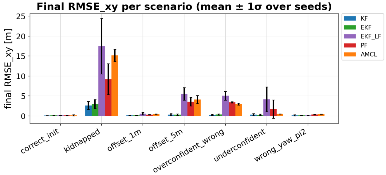
Fig. 3: Final RMSE_{xy} per scenario (mean \pm 1\sigma , ten seeds). The landmark filters (KF, EKF) remain low across every adverse scenario; the scan filters explode under offset_5m , overconfident_wrong , and kidnapped .
