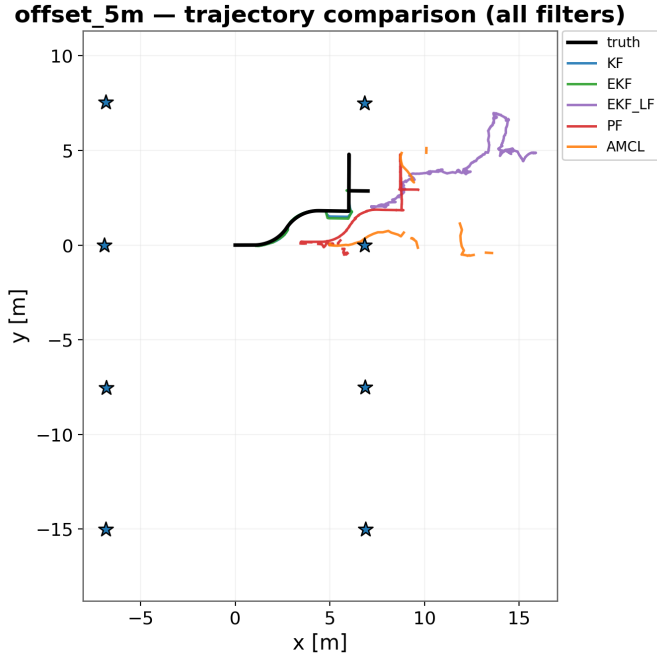
Fig. 3: Estimated trajectories under a 5 m wrong start. The landmark filters (KF, EKF) lock onto the true path (black); the scan filters (EKF-LF, PF, AMCL) drift away into a wrong but symmetric bay. Stars mark the AprilTag landmarks.
