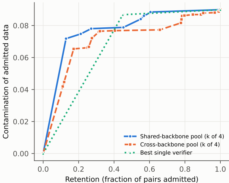
Retention and contamination frontier, eta = 10%
