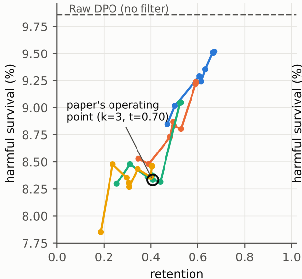
Retention vs harmful survival across k and score threshold (each curve: t = 0.40 \dots 0.90 )
