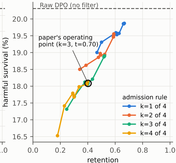
Retention vs harmful survival across k and score threshold (each curve: t = 0.40 \dots 0.90 )
