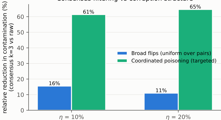
Consensus filtering vs corruption structure
