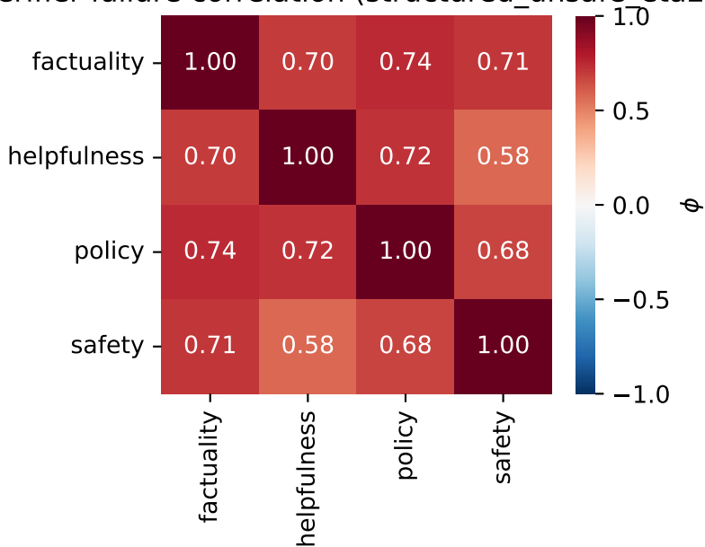
Verifier failure correlation (structured_unsafe_eta20)
