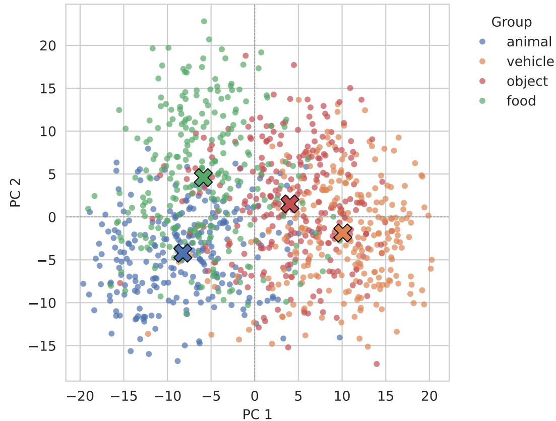
Feature Space by Semantic Group - base Separation: 1.05 (inter=3.72, intra=3.55)
