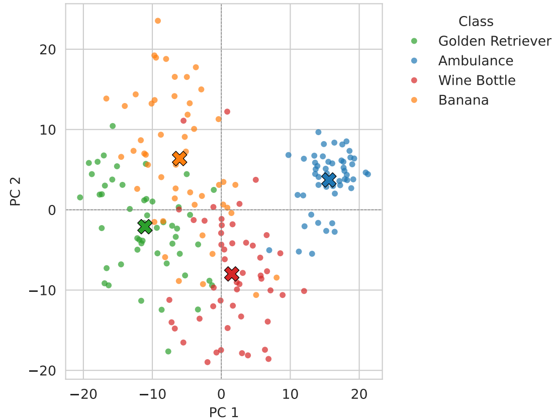
Feature Space (PCA) - base Separation: 1.09 (inter=3.70, intra=3.39)
