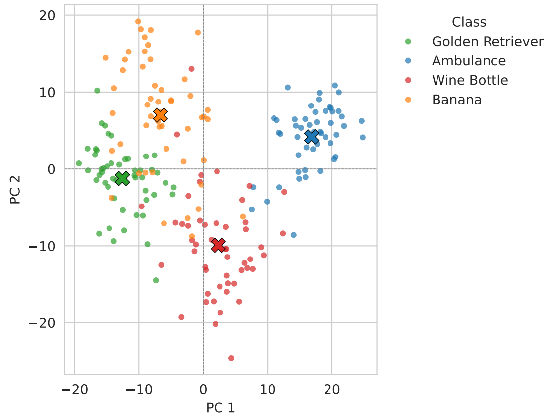
Feature Space (PCA) - cm-strong Separation: 1.11 (inter=4.16, intra=3.74)
