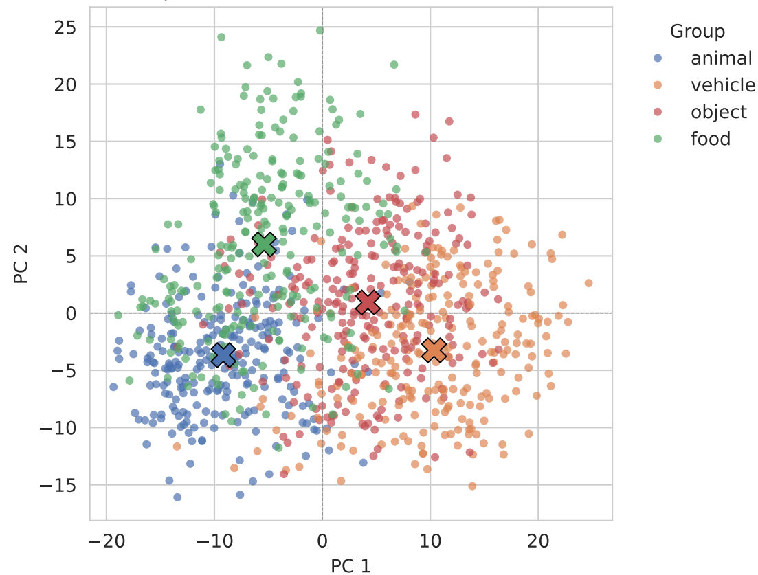
Feature Space by Semantic Group - crop Separation: 1.05 (inter=4.36, intra=4.15)
