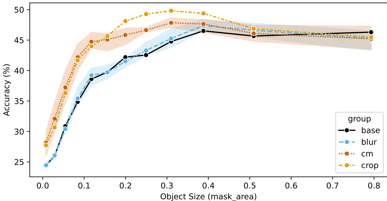
Accuracy vs Object Size
