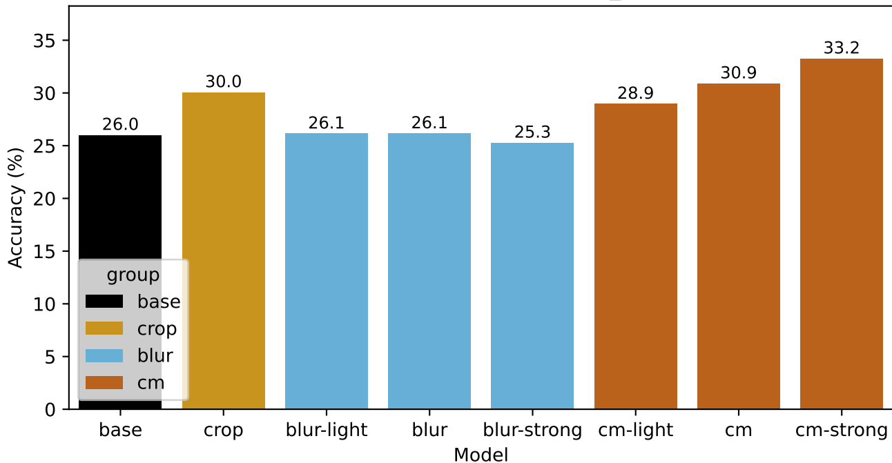
Performance on Small Objects (mask_area \leq 0.05 )
