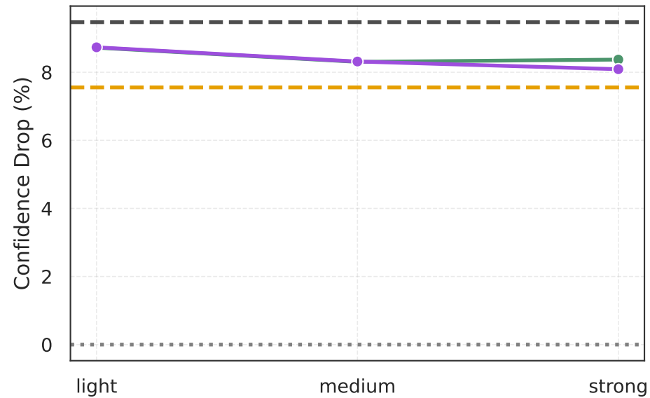
Correct Predictions
