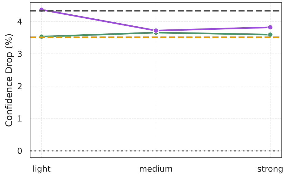
Incorrect Predictions
