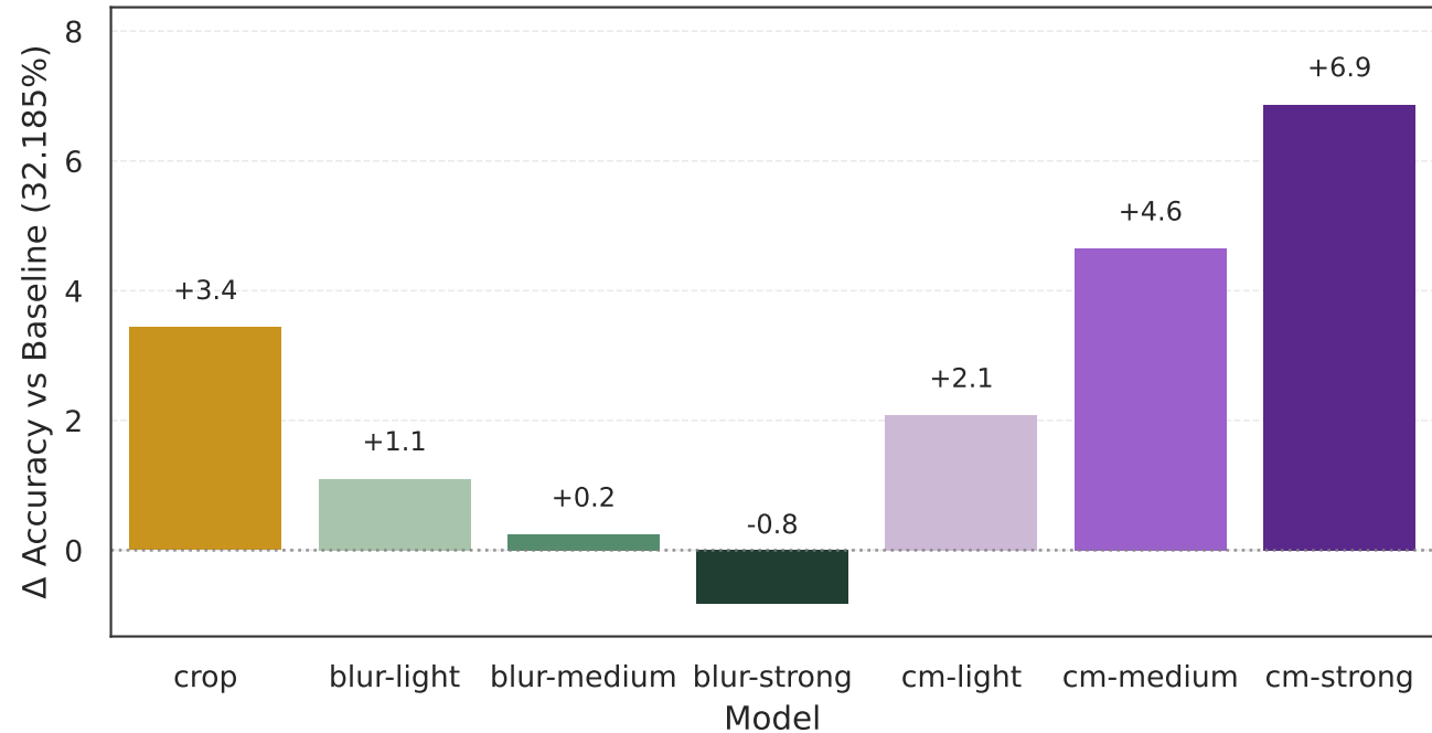
Performance on Small Objects (Rel. Mask Area \leq 0.132 )
