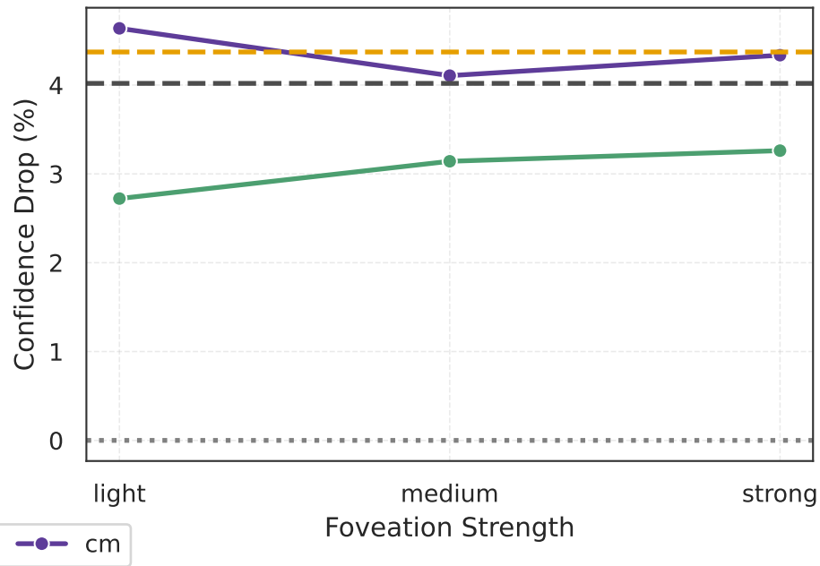
Incorrect Predictions
