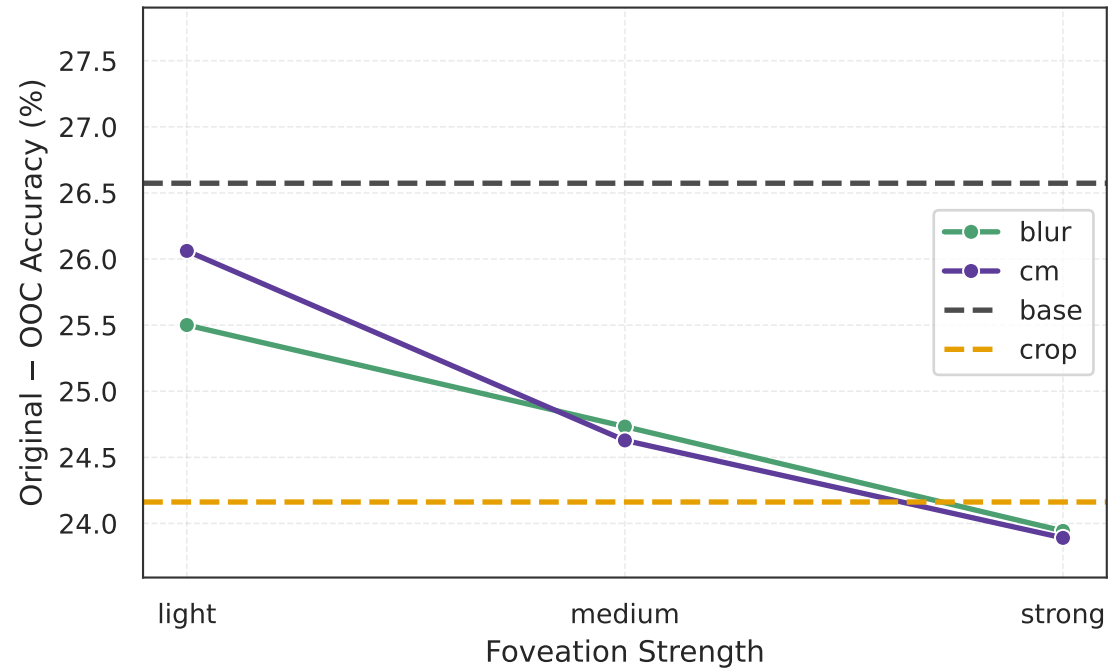
Original vs OOC Gap
