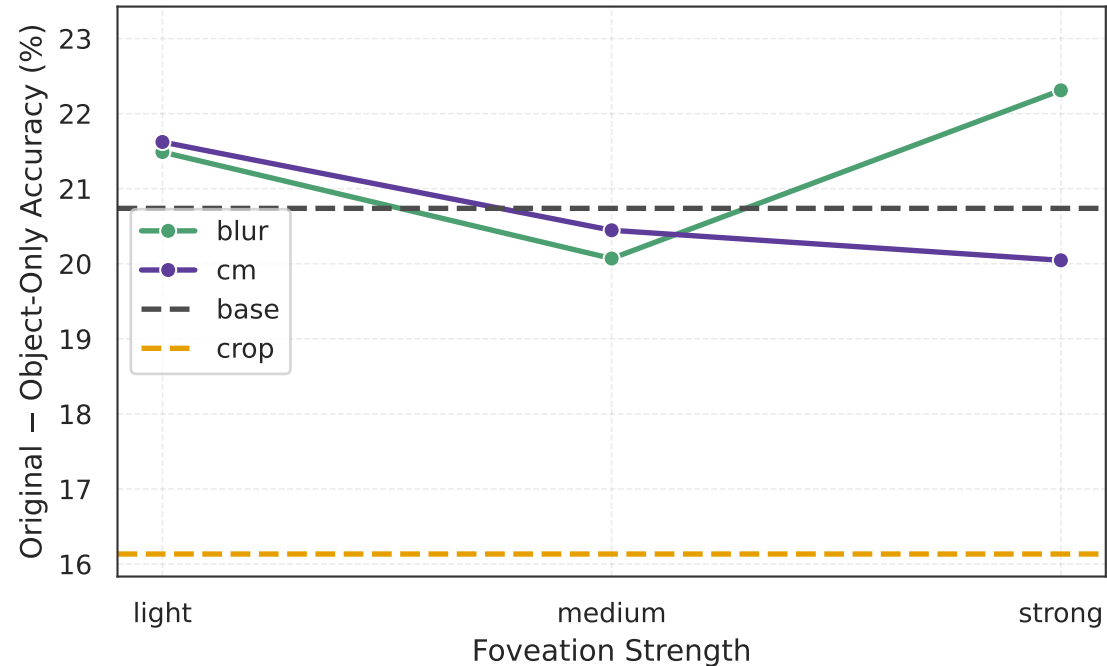
Original vs Object-Only Gap
