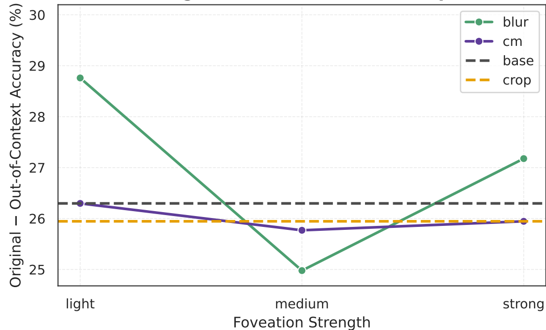
Original vs Out-of-Context Gap
