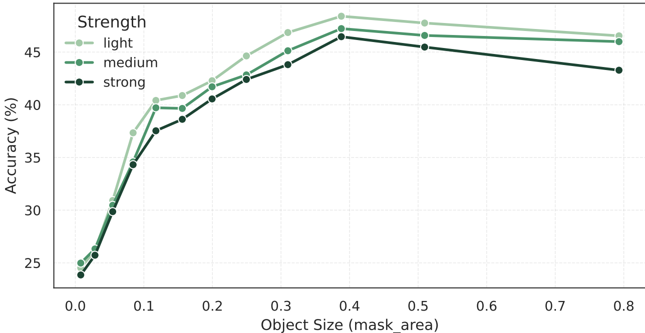
BLUR - Accuracy vs Object Size
