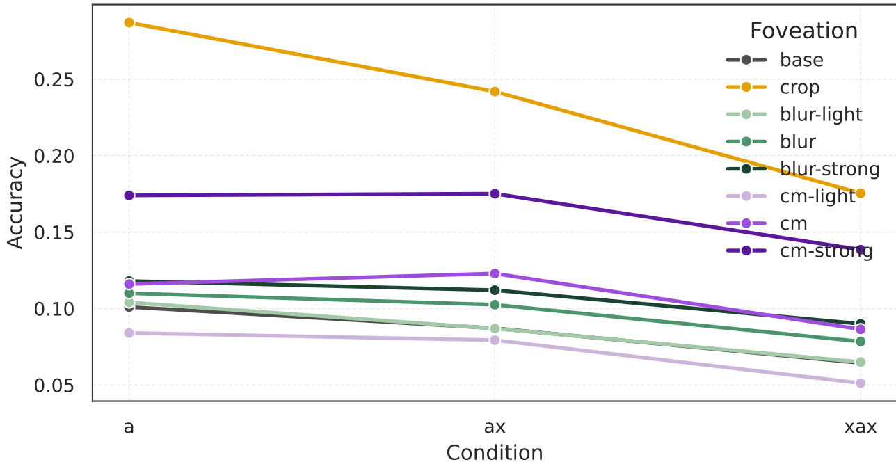
Accuracy Trend at Distance = 20
