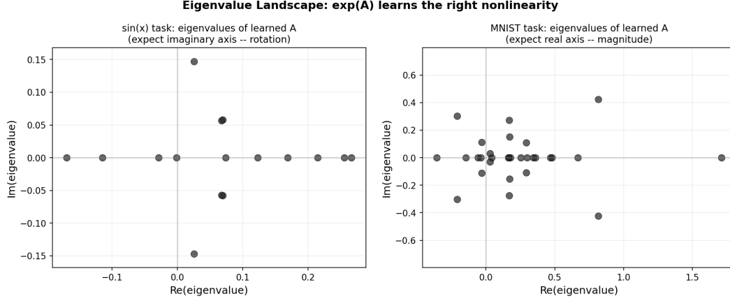
Figure 20: Eigenvalue landscape comparison between tasks. Left: \sin(x) task, where eigenvalues cluster near the imaginary axis (rotation-dominated, as expected for periodic structure). Right: MNIST task, where eigenvalues spread along the real axis (magnitude-dominated, reflecting classification’s reliance on feature scaling). The task geometry determines which mode of \exp(A) the network exploits.
