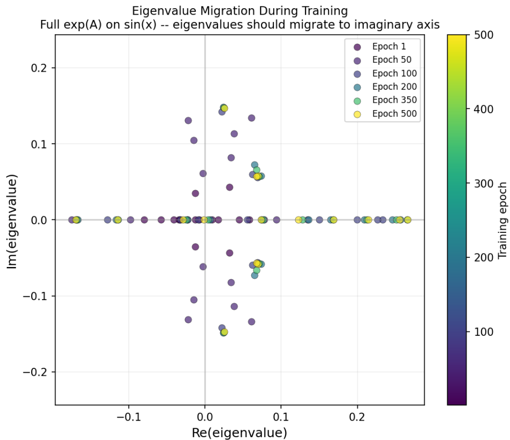
Figure 19: Eigenvalue migration during training on \sin(x) (full \exp(A) , 8 layers). Eigenvalues begin near the real axis (epoch 1, dark) and migrate toward the imaginary axis (epoch 500, bright), developing the conjugate pairs needed for sinusoidal representation. The network discovers rotational structure autonomously.
