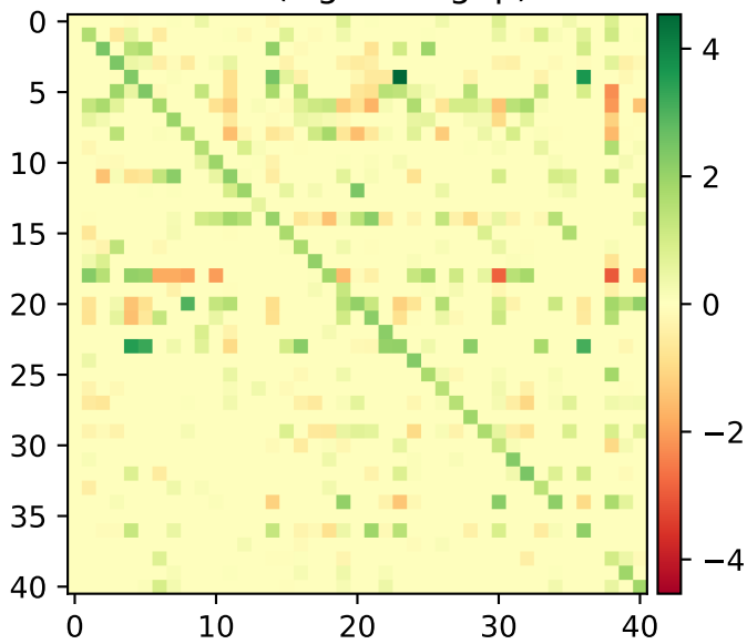
Targets of Col4a2
