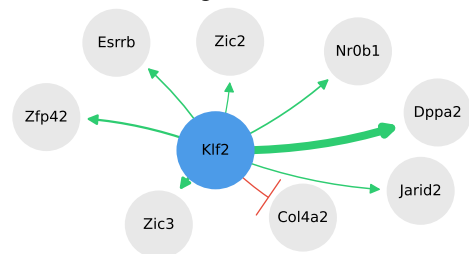
Targets of Klf2
