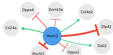
Targets of Hoxb2
