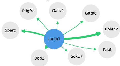
Targets of Lamb1
