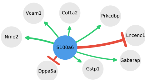
Targets of S100a6
