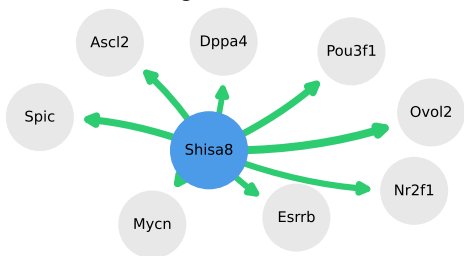
Targets of Shisa8
