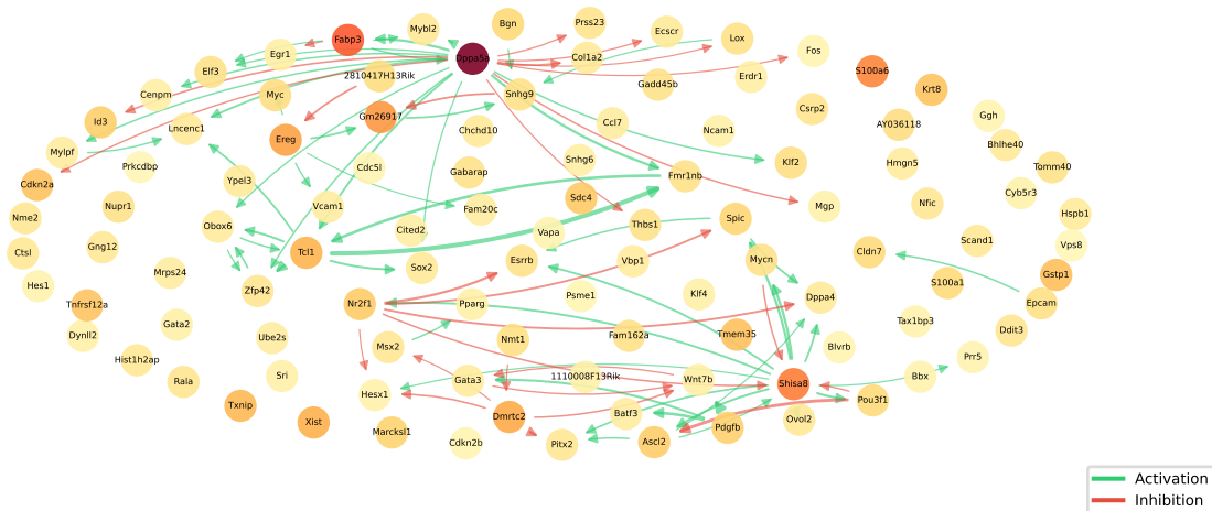
B GRN (signed log1p)
