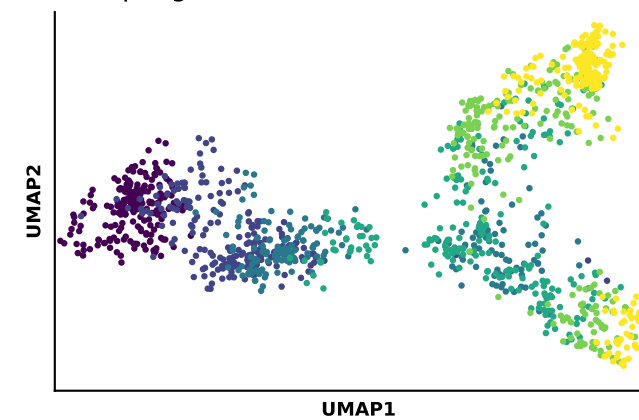
C Sampling theta
