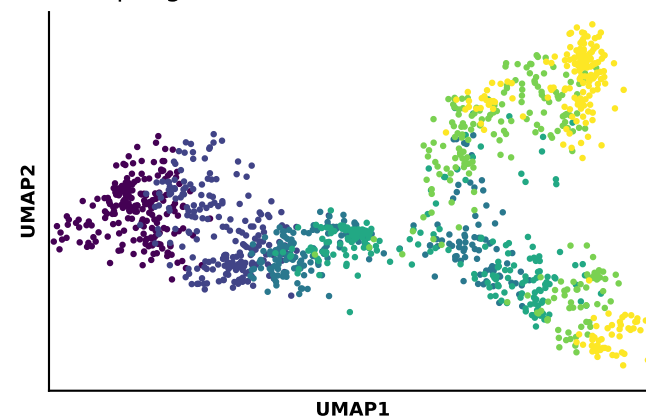
B Sampling beta
