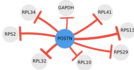
Targets of POSTN
