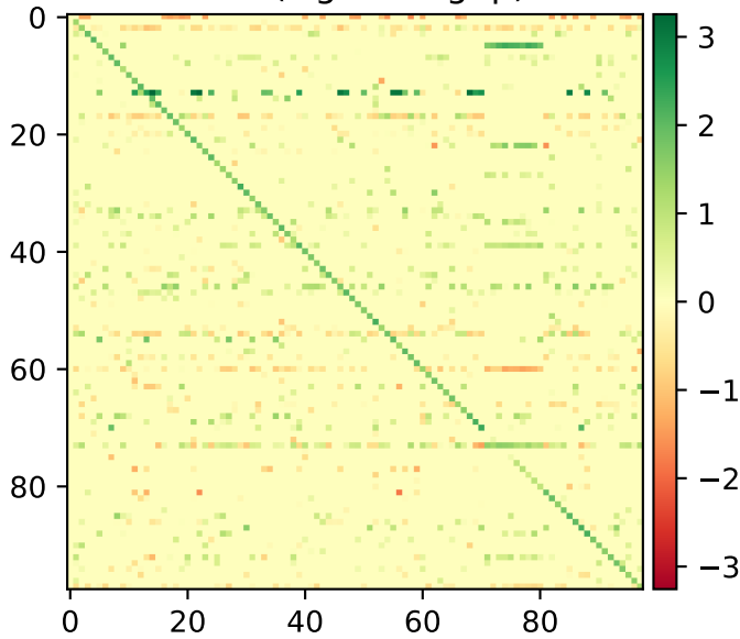
Targets of CHGA
