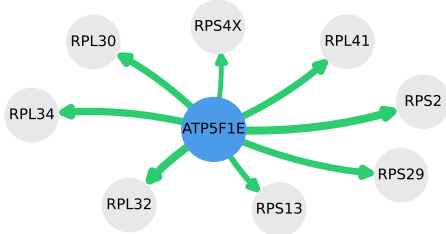
Targets of ATP5F1E
