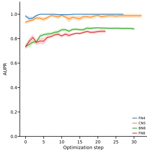
B AUPR over training
