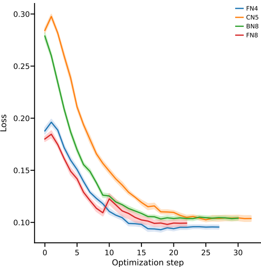
A Training loss
