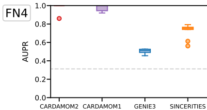
A Snapshot-based
