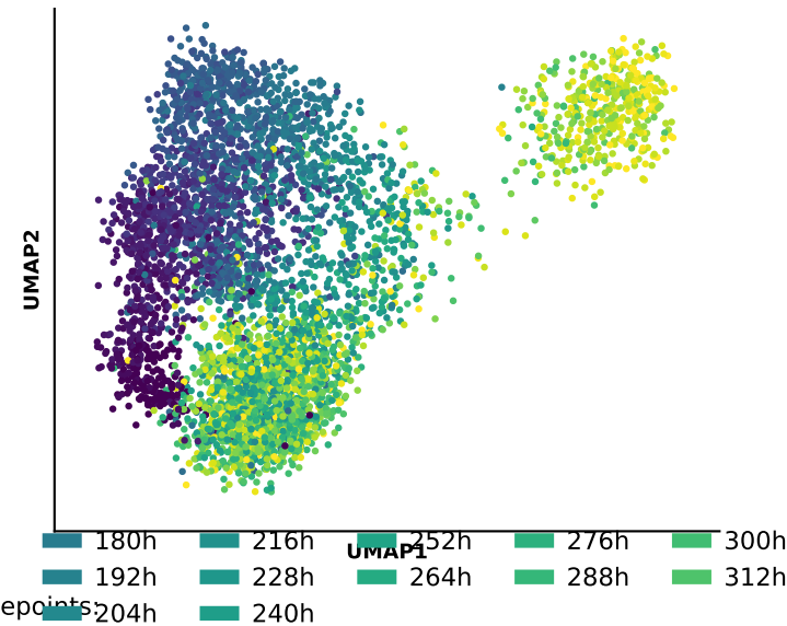
C Sampling theta
