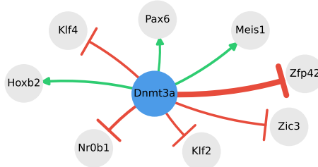
Targets of Dnmt3a
