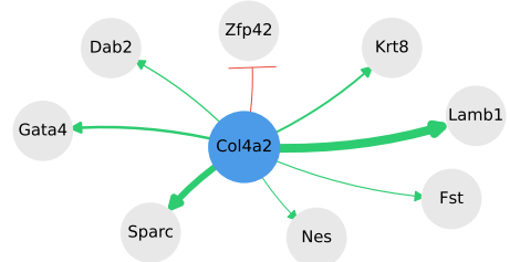
Targets of Col4a2
