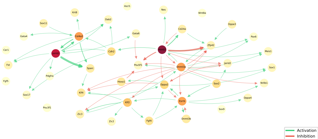
B GRN (signed log1p)
