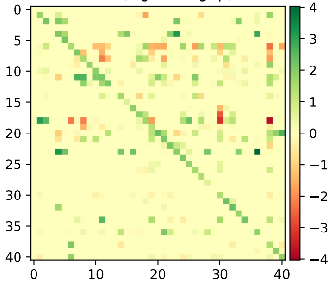
Targets of Hoxb2
