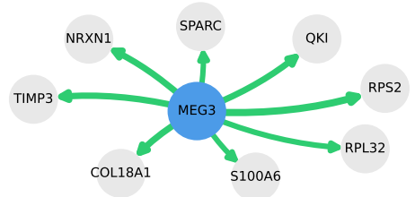
Targets of MEG3
