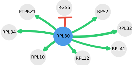
Targets of RPL30
