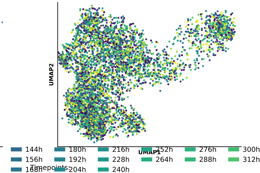
C Sampling theta
