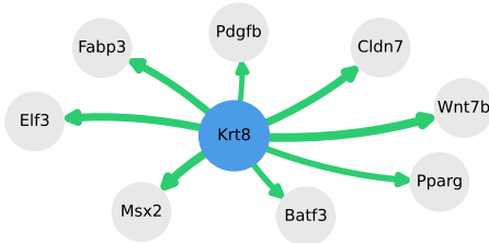
Targets of Krt8
