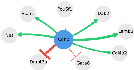
Targets of Cdh2
