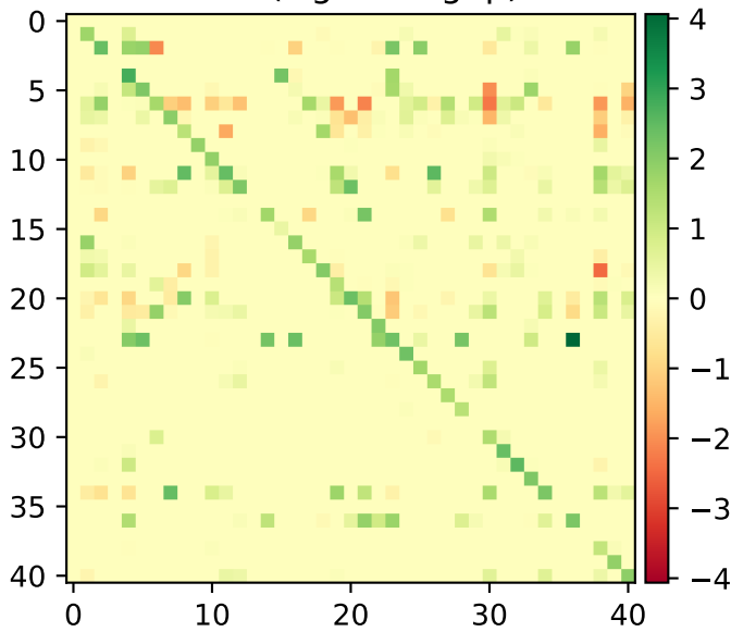
Targets of Lamb1
