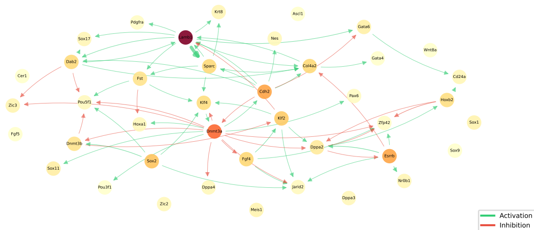
GRN (signed log1p)
