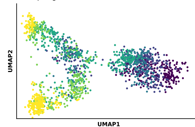
C Sampling theta
