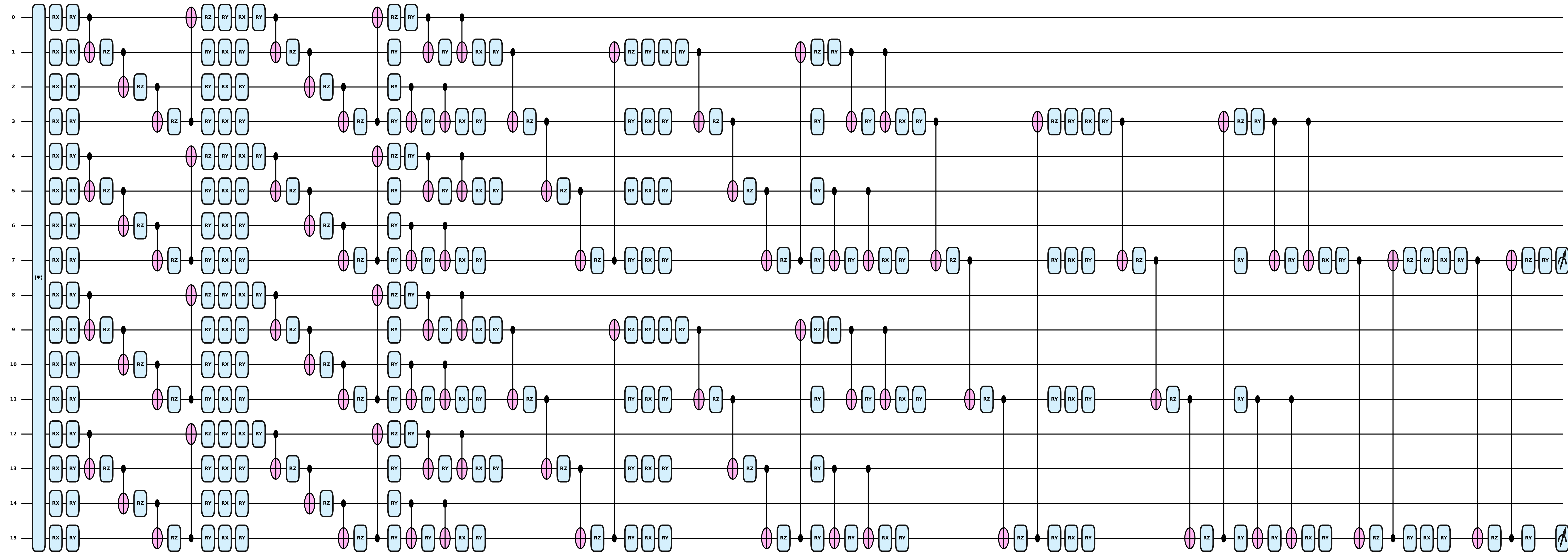
Architecture LD-QCNN (16 qubits, k=4, depth=2)
