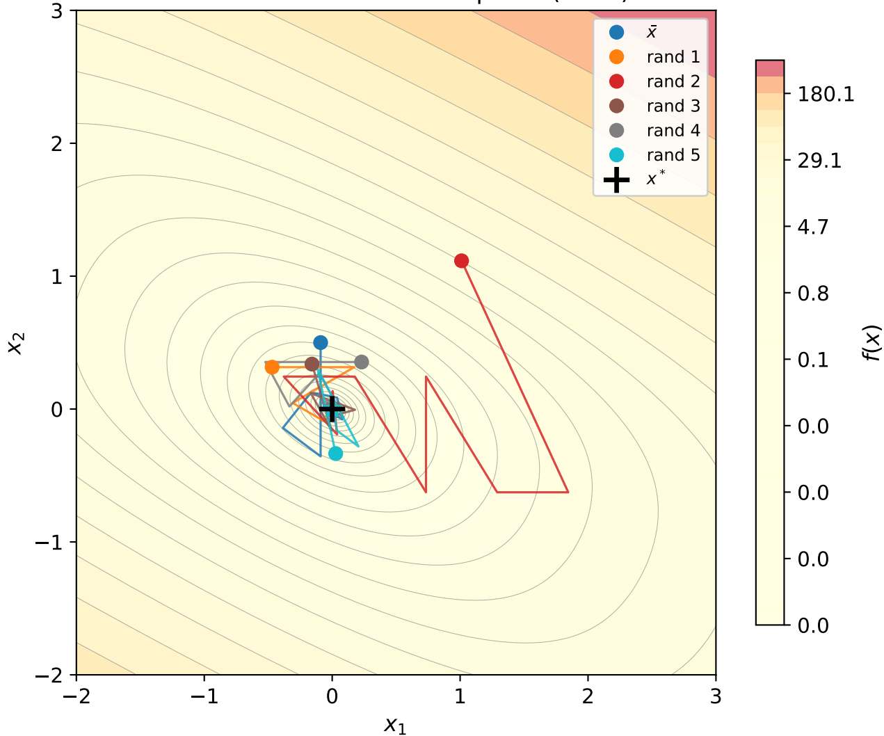
Zakharov — Nelder-Mead paths ( n = 2 )
