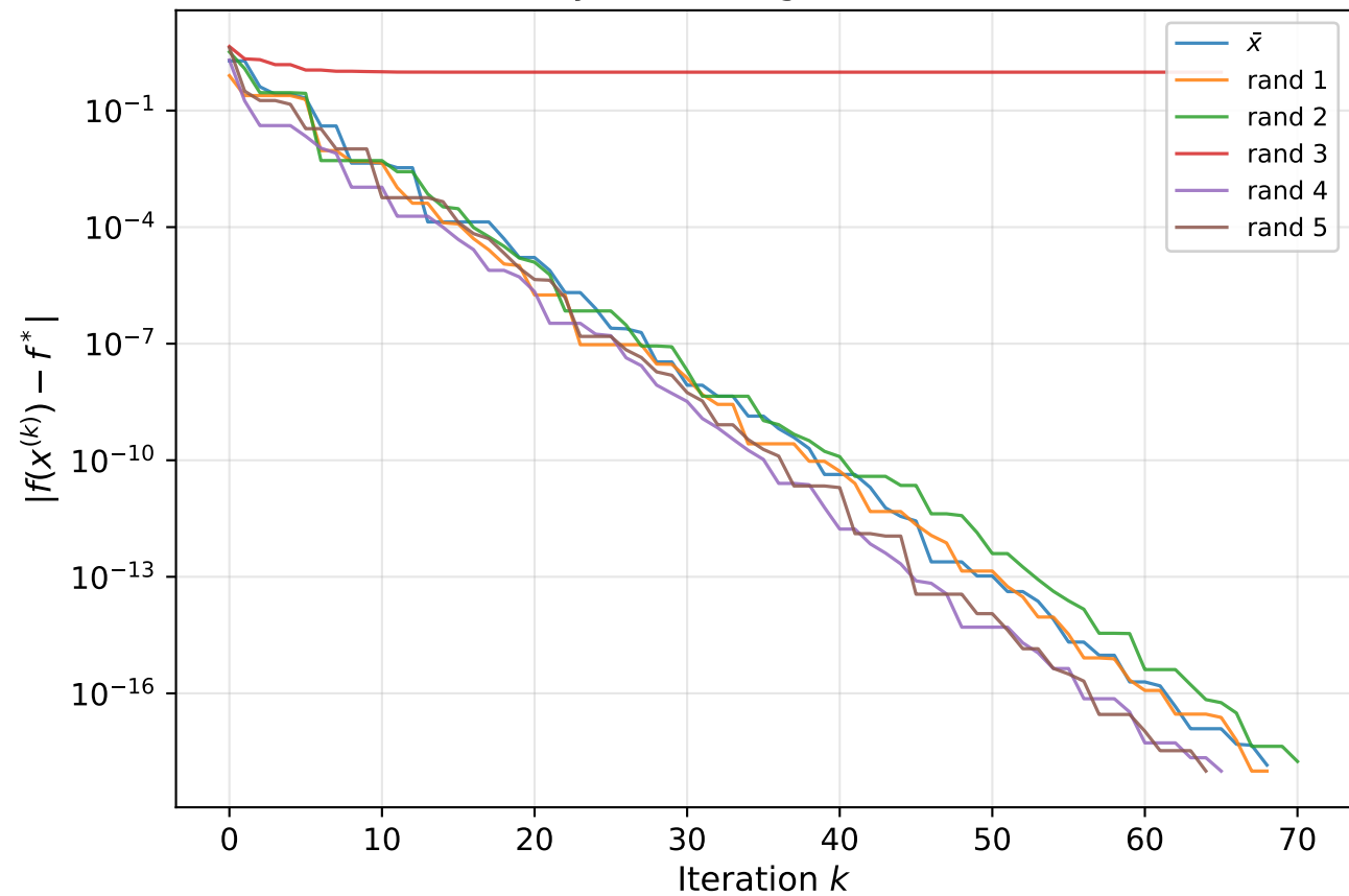
Levy — convergence ( n = 2 )
