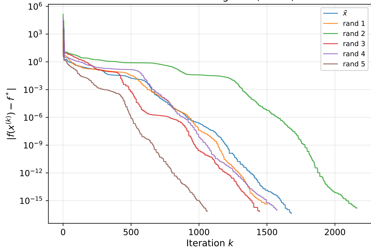
Zakharov — convergence ( n = 10 )
