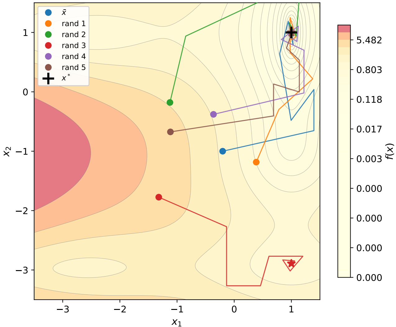
Levy — Nelder-Mead paths ( n = 2 )
