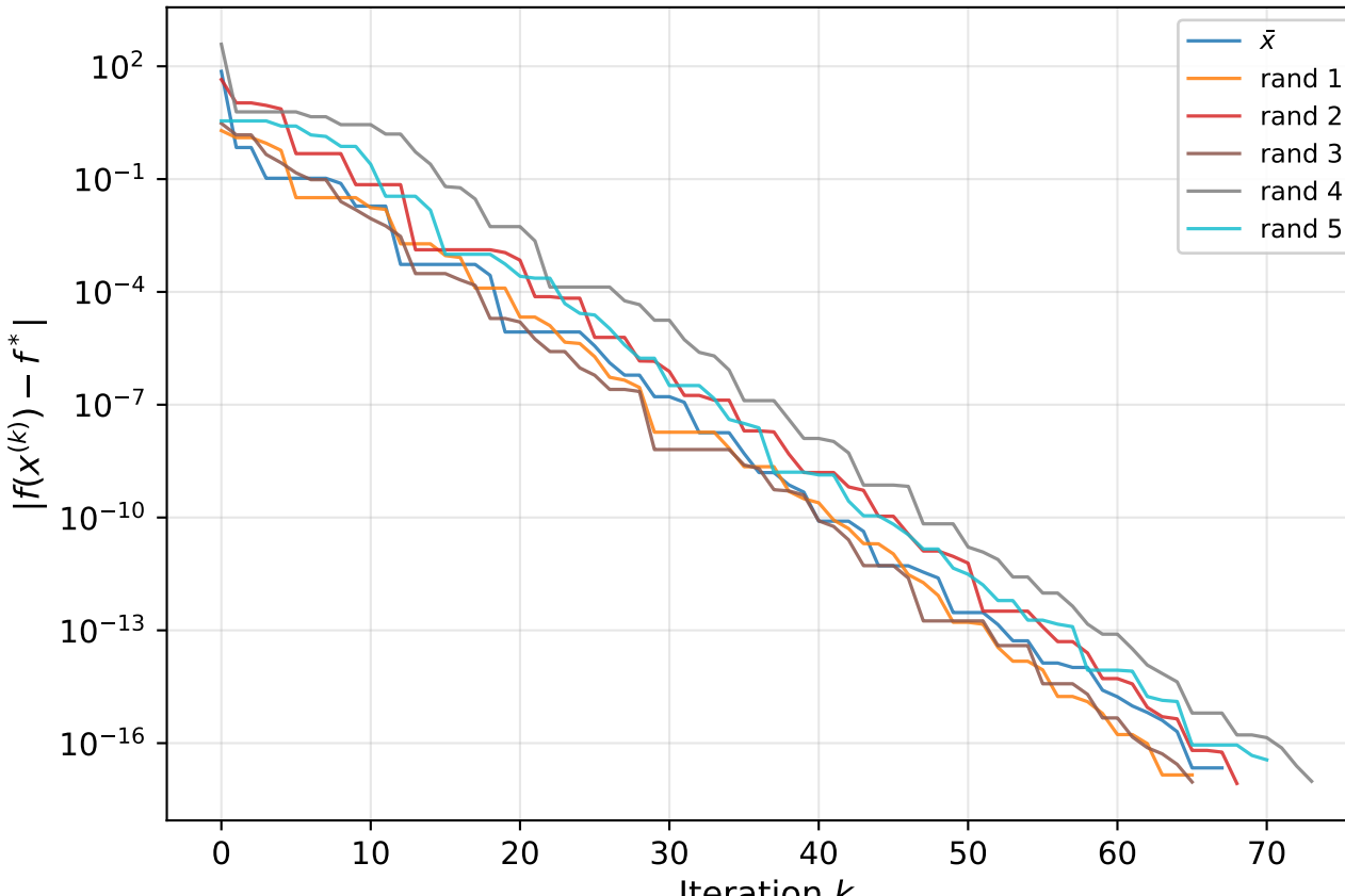
Dixon-Price — convergence ( n = 2 )
