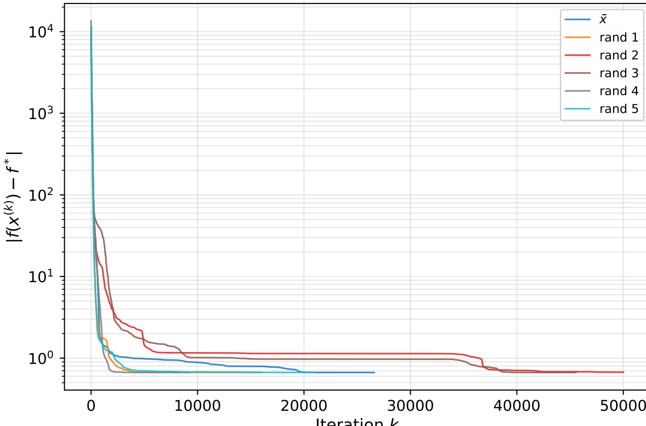
Dixon-Price — convergence ( n = 20 )
