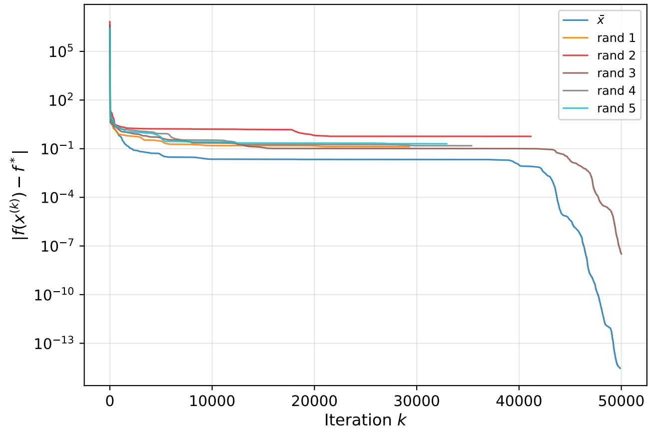
Zakharov — convergence ( n = 20 )
